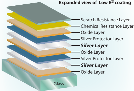
Expanded view of Low E 2 coating
